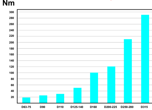
KELEBEK VANA TORK DİYAGRAMI BUTTERFLY VALVE TORQUE GRAPH
