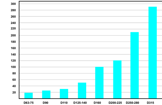
KELEBEK VANA TORK DİYAGRAMI BUTTERFLY VALVE TORQUE GRAPH
